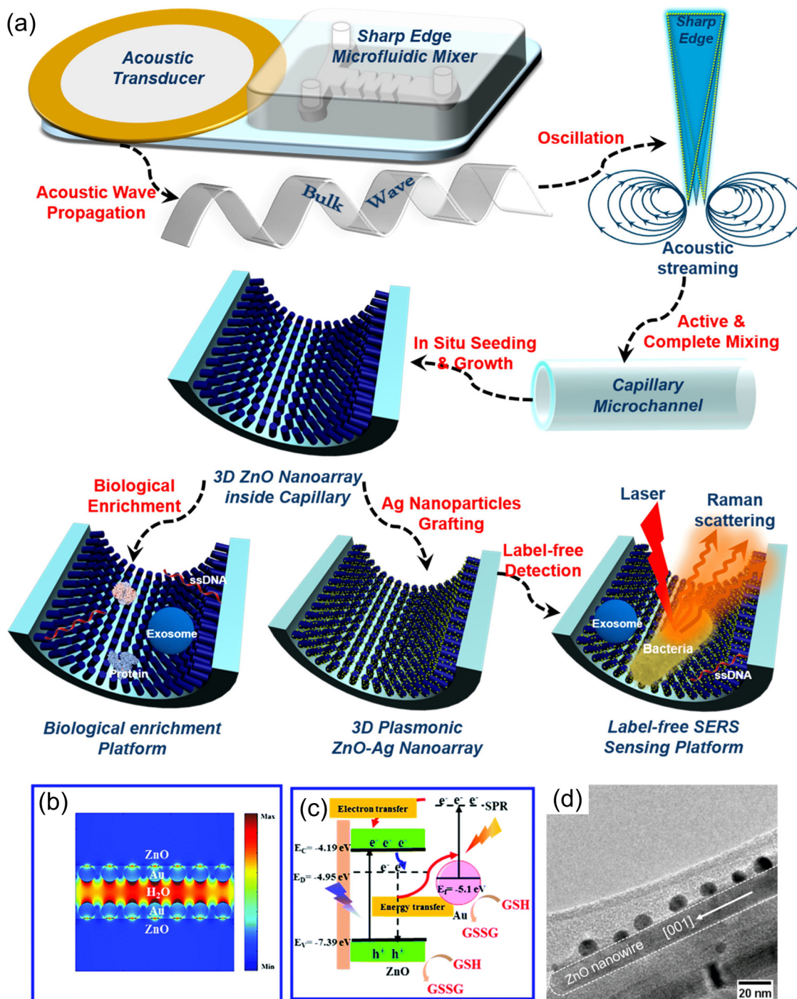
Fig. 3 (a) Acoustofluidic driven synthesis of ZnO NRs/Ag NPs microfluidic SERS platform for detecting various biological elements. Copyrights ACS Publications 2020. 154 (b and c) FDTD simulation of the electromagnetic field modulation in ZnO NRs/Au NPs for photoelectrochemical detection of glutathione. Proposed electron transfer mechanism along with the obtained metal–semiconductor interface. Copyrights RCS Publishing 2019. 118 (d) Pb acetylene electric detection employing Au decorated ZnONWs. Copyrights ACS Publications 2020. 160
