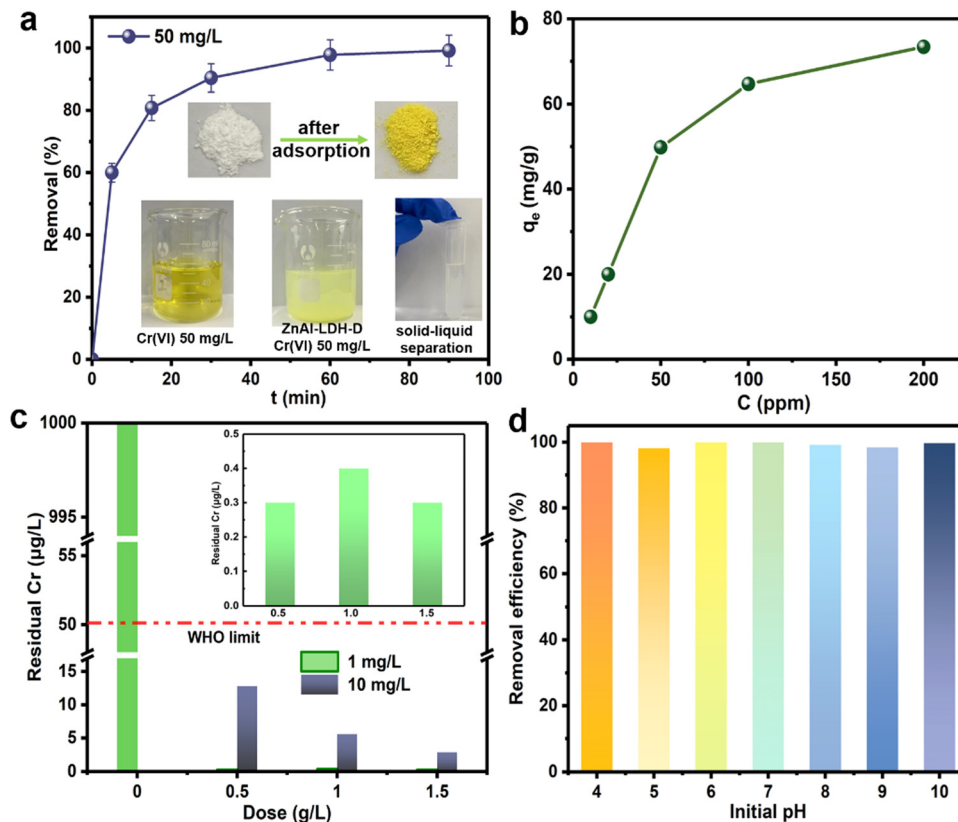
Fig. 4 (a) Sorption kinetics of \text{Cr}^{\text{VI}} by ZnAl-LDH-D (dose = 0.5 g \text{L}^{-1} , C_0 = 50 \text{ mg L}^{-1} ); (b) sorption isotherms of \text{Cr}^{\text{VI}} by ZnAl-LDH-D (dose = 0.5 g \text{L}^{-1} , C_0 = 10\text{--}200 \text{ mg L}^{-1} , t = 2 \text{ h} ); (c) deep adsorption performance of ZnAl-LDH-D toward \text{Cr}^{\text{VI}} with a low concentration ( t = 2 \text{ h} ); (d) influence of the initial pH on the adsorption performance (dose = 0.5 g \text{L}^{-1} , C_0 = 50 \text{ mg L}^{-1} , t = 2 \text{ h} ).
