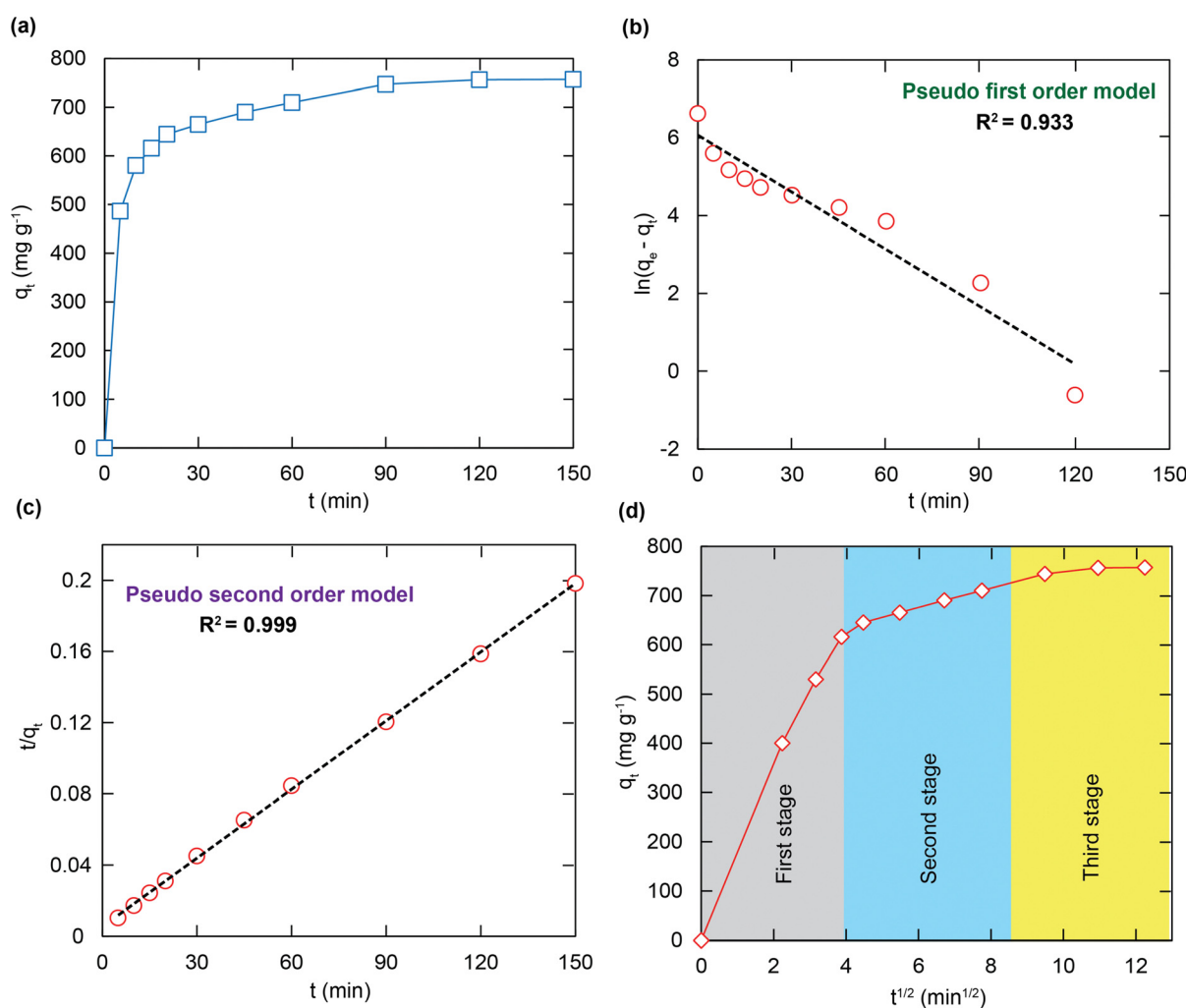
Fig. 6 The kinetic curve for the adsorption of RhB onto H + ⊂BUT-8(Cr) [ m = 10 mg, V_{\text{RhB}} = 100 mL, C_0 = 100 mg L -1 , pH = 3] (a); data fitting with the adsorption kinetic models: pseudo first order (b), pseudo second order (c) and intra-particle diffusion model (d).
