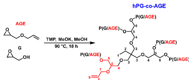
Scheme 1 Synthesis of hPG-co-AGE.
