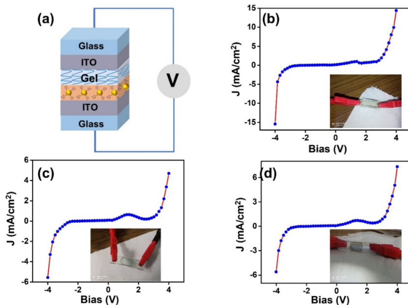
Fig. 6 (a) Schematic representation of device fabrication for I-V measurements, (b)–(d) applied voltage vs. current density plots of Ag NPs, L-Cys@Ag, and D-Cys@Ag NPs, respectively. Inset images show photographs of actual devices.
