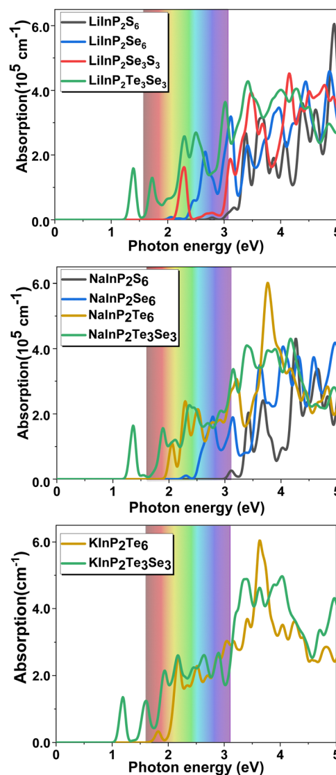
Fig. 3 Absorbance of AMInP 2 X 3 Y 3 monolayers computed using the G 0 W 0 + BSE method for the light incidence in-plane (XY) direction. The iridescent colors mark the visible spectrum.
