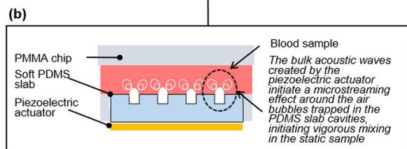
Fig. 1 A finger-actuated filtered blood lysate preparation device. (a) Isometric CAD view of the concept, illustrating seven functional elements. (b) Illustration of the acoustic mixing principles developed in ref. 11.
