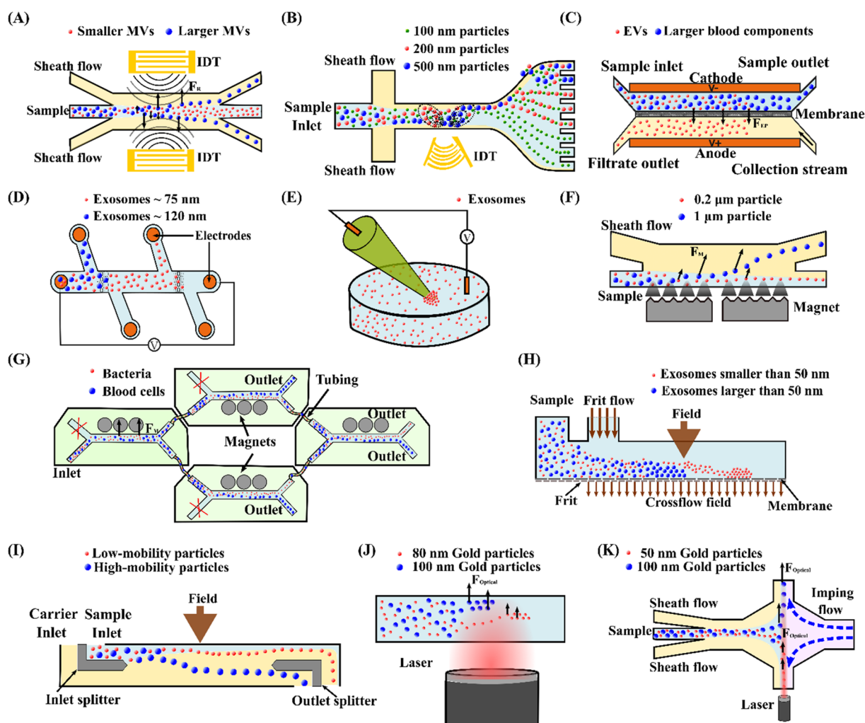
Fig. 3 Active microfluidic techniques for manipulation, focus, and separation of submicron and nanoparticles. (A) Separation of MVs by acoustophoresis. 103 (B) Focused TSWA device for separating 100 nm, 200 nm and 500 nm polystyrene particles. 82 (C) Isolation EVs from whole blood by DC electrophoresis. 115 (D) Simultaneous capture and separation of different subpopulations of exosomes by DC insulator-based dielectrophoresis. 137 (E) Entrapment of exosomes by a low voltage nanopipette DEP device. 76 (F) Separation of 0.2 μm and 1 μm fluorescence polystyrene particles by magnetophoresis. 146 (G) Separation of bacteria by integrating multiple magnetophoresis devices. 2 (H) Size fractionation of exosomes by field-flow fractionation. 166 (I) SPLITT device for improved fractionation of cells/particles. 168 (J) Trapping of 80 nm and 100 nm gold particles by optofluidics. 176 (K) Optofluidic sorting of gold nanoparticles of 50 nm and 100 nm diameters. 172
