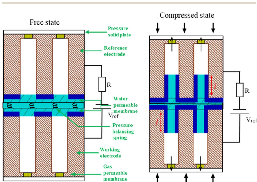
Fig. 7 A sketch of the current-generating porous electrode. V_{ref} denotes the bias voltage between the counter and working electrodes. The applied pressure forces the electrolyte inside the pores and increases the contact area between the electrode and electrolyte, with the corresponding formation of double layers, depicted in dark blue colour. Moving the piston up and down will change the double-layer capacitance and trigger the current into and from the electrode. Pores can be of any shape, e.g. slit or cylindrical, but with smooth surfaces not causing the hysteresis in the forward and backward motion of the liquid. The spring must be stiff enough not to delay the response to the external pressure.
