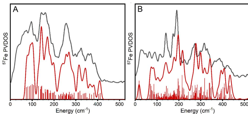
Fig. 4 (A) Calculated P-cluster PVDOS from the MoFe QM/MM model, BS-1247, (red line) compared to the experimental apo-MoFe PVDOS (black). Calculations were performed using a 39 atom QM-region/Hessian. (B) Overlay of calculated FeMoco (red, solid) vs. derived experimental FeMoco (black, solid) PVDOS. Individual calculated modes and their intensities are represented as bars, while the solid line represents the 12 \text{cm}^{-1} FWHM broadened composite PVDOS. Calculations were performed considering 247 atoms in the QM-region/Hessian and a BS7-235 broken-symmetry solution.
