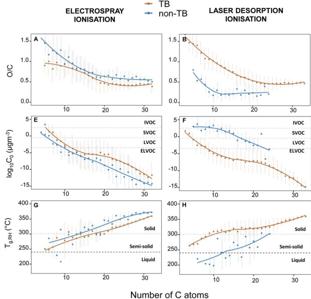
Fig. 5 Average values of O/C, \log_{10} of estimated saturation mass concentration ( \log_{10}C_0 ), and relative-humidity dependent glass transition temperature ( T_{g,RH} ) against the number of C atoms in the formulae assigned. Components exclusively identified in BBAug1318 (TB-rich) are plotted relative to non-TB components (identified in BBAug1011, BBAug0910 (NT), and/or BBAug09 (DT)). In (–)ESI, all three non-TB aerosol samples were considered, while for (–)LDI, non-TB refers to BBAug0910 (NT) and BBAug1011 only.
