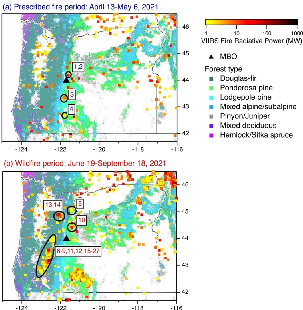
Fig. 2 Fire hotspots in Oregon between (a) April 13 and May 6, 2021, and (b) June 19 and September 18, 2021, colored by their VIIRS fire radiative power (FRP). Note the log scale of the FRP coloring. Suspected source fires are circled and labeled by event number. Note that the circles sometimes include more than one fire. The black triangle shows the location of MBO. Forest type data from the US Forest Service National Forest Type Dataset. 85
