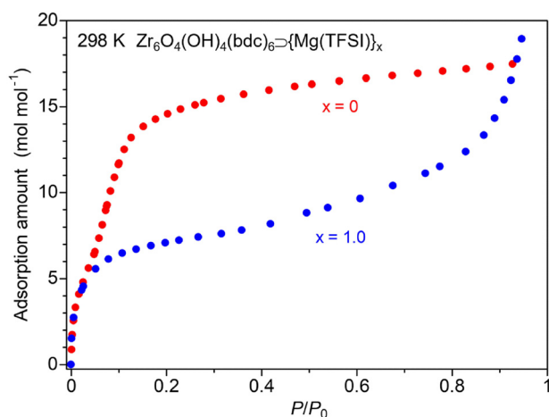
Fig. 4 Adsorption isotherms of blank UiO-66 ( x = 0 ) and \text{UiO-66} \supset \{\text{Mg}(\text{TFSI})_2\}_{1.0} ( x = 1.0 ) under MeOH vapor.
