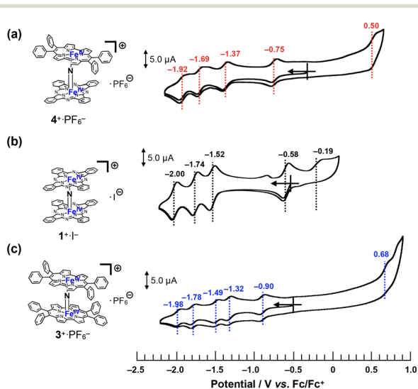
Fig. 5 Comparison of cyclic voltammograms of (a) 4^+\cdot\text{PF}_6^- , (b) 1^+\cdot\text{I}^- , and (c) 3^+\cdot\text{PF}_6^- in a pyridine solution containing 100 mM of ^n\text{Bu}_4\text{N}^+\cdot\text{PF}_6^- at room temperature. [Substrate] = 200 \mu\text{M} , [scan rate] = 100 \text{mV s}^{-1} .
