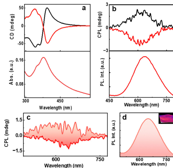
Fig. 4 (a) CD and the corresponding UV-visible spectra and (b) CPL and the corresponding PL spectra of aqueous AuNC solution. Black and red traces correspond to D- and L-AuNCs, respectively. (c) CPL and the (d) luminescence plot of the AuNC incorporated PVA film. The positive and negative CPL plot corresponds to D- and L-AuNC, respectively. The inset in 'd' shows the photograph of the film under 365 nm UV illumination.
