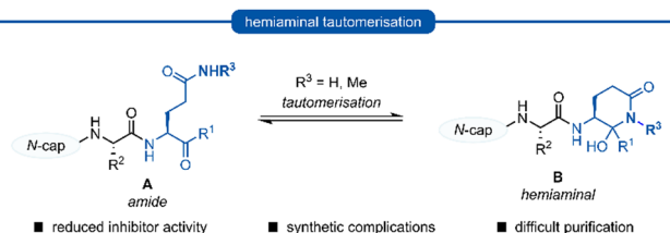
Scheme 1 Generalised formation of hemiaminal B via tautomerisation of P 1 glutamine inhibitors A onto the electrophilic warhead.
