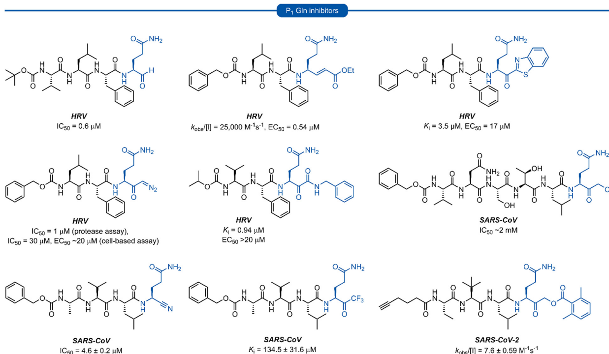
Fig. 2 Representative 3C/3CL PRO inhibitors possessing a P 1 (L)-glutamine residue with various electrophilic warheads.
