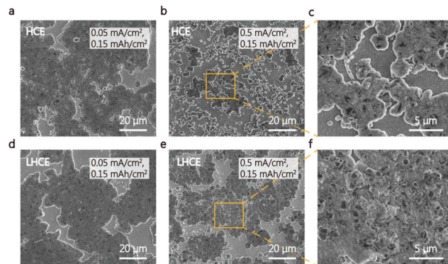
Fig. 4 Top-view SEM images of K deposition morphologies in (a–c) HCE and (d–f) LHCE with enlarged views (c and f) at a current density of (a and d) 0.05 mA cm -2 and (b and e) 0.5 mA cm -2 with a capacity of 0.15 mA h cm -2 .
