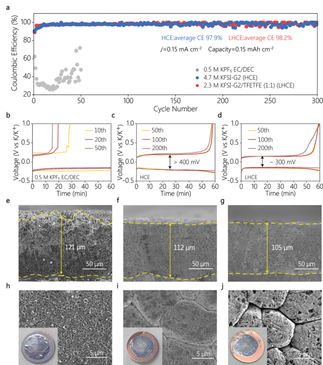
Fig. 3 (a) Cycling performances of K/Cu coin cells and the corresponding voltage profiles in (b) 0.5 M KPF 6 EC/DEC electrolyte, (c) HCE and (d) LHCE at 0.15 mA cm -2 . (e–g) Cross-sectional and (h–j) top-view SEM images of K deposition morphologies in (e and h) 0.5 M KPF 6 EC/DEC, (f and i) HCE and (g and j) LHCE. Optical images of K deposits on Cu foil are shown in the inset of h–j. The capacity of K metal on the Cu substrate was 4.0 mA h cm -2 .
