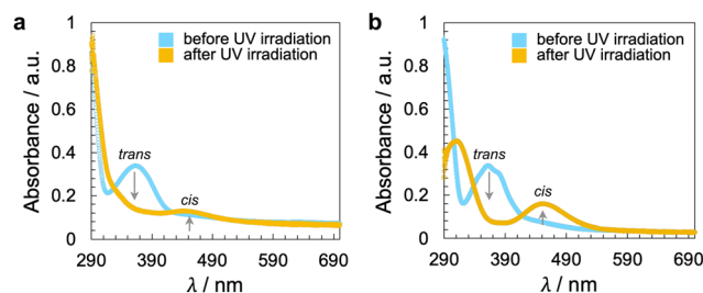
Fig. 5 UV-vis spectra of the CNCs in DMF (20 °C) before and after illumination with UV light at \lambda = 365 nm for a time period of t = 10 s: (a) CNC-AC and (b) CNC-AB. Longer exposure, up to t = 60 s, did not lead to a discernible change in the spectra, and thus, all azobenzene pendants are already in the cis configuration in solution after a t = 10 s exposure to UV light (ESI,† Fig. S16).
