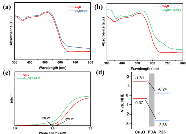
Fig. 6 The UV-vis diffuse reflectance spectra of (a) \text{Cu}_2\text{O} and \text{Cu}_2\text{O}/\text{PDA} and (b) \text{Cu}_2\text{O} and \text{Cu}_2\text{O}/\text{PDA}/\text{P25} , (c) Tauc plots, and (d) schematic diagram of charge transfer between \text{Cu}_2\text{O} and P25.
