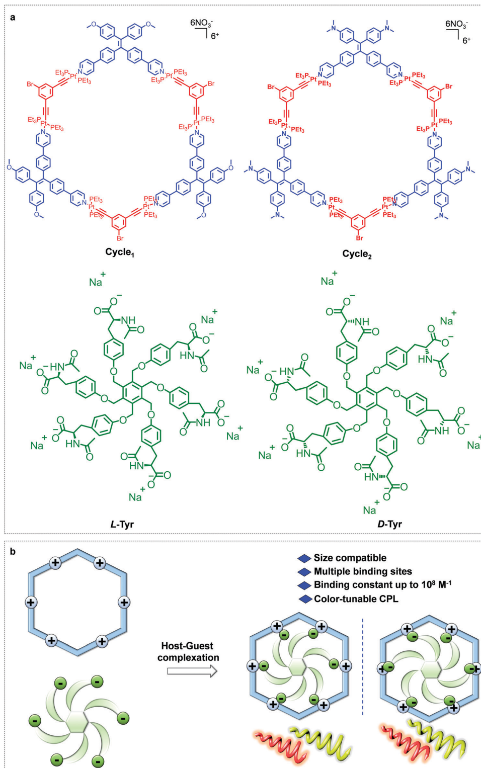
Scheme 1 (a) Chemical structures of the metacycles and guests. (b) Highly affiliative host–guest complexation.
