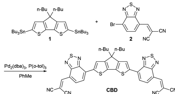
Scheme 1 Synthetic route for the small molecule CBD .
