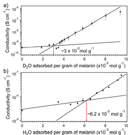
Fig. 11 (A) Conductivity of melanin with \text{D}_2\text{O} content. (B) Conductivity of melanin with \text{H}_2\text{O} content. Red arrows (with values) indicate the upturn in the conductivity at a critical amount of water content. Reprinted with permission from S. B. Riener et al. J. Phys. Chem. B , 2015, 119 , 14994–15000. Copyright 2015 American Chemical Society. 46
