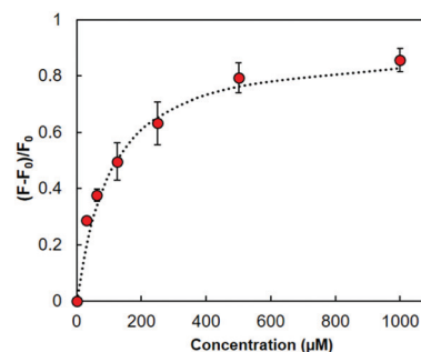
Fig. 2 Changes in relative fluorescence intensity at 468 nm in HOLO(FSA)(MBA) upon the addition of cephalexin ( \lambda_{\text{ex}} = 365 \text{ nm} ). The correlation factor of the fitting curve (dashed line) was 0.98.
