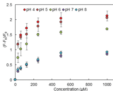
Fig. 3 Changes in relative fluorescence intensity in HOLO(FSA)(MBA) on binding cephalexin in aqueous media at different pH values.
