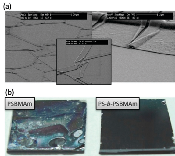
Fig. 2 (a) Scanning electron microscopy pictures displaying the detachment of poly(poly(ethylene glycol) methacrylate) (PEGMA) brushes grafted from SiOx substrates using silane chemistry, after 7 days of immersion in a cell culture medium at 37 °C (reprinted with permission from ref. 76. Copyright 2008 American Chemical Society). (b) photos displaying the detachment of poly(sulfobetaine methacrylamide) (SBMAm) brushes grafted from silicon wafers via silane linkers (left), after immersion for 3 months in seawater and the prevention of this detachment by utilisation of diblock copolymer brushes (see also Section 3.2) (reprinted with permission from ref. 141. Copyright 2013 American Chemical Society).
