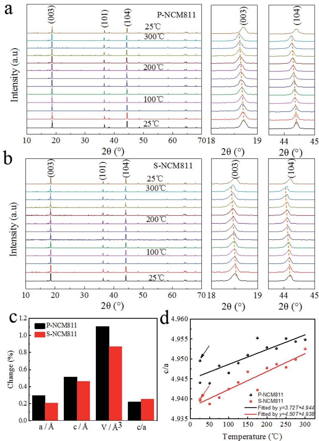
Fig. 2 In situ XRD of (a) P-NCM811 and (b) S-NCM811 cathode materials. Detailed 2\theta degree ranges of 18.0–19.0 ^\circ and 43.5–45 ^\circ are also displayed. (c) Lattice and volume change. (d) The change of c/a with the increment of the temperature.
