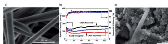
Fig. 6 (a) SEM images of CADS nanowires, (b) cycle life of CADS micropillars, CADS microwires, and CADS nanowires, (c) SEM images of CADS nanowires after 100 cycles. The figures are reproduced from ref. 64 with permission. © American Chemical Society.
