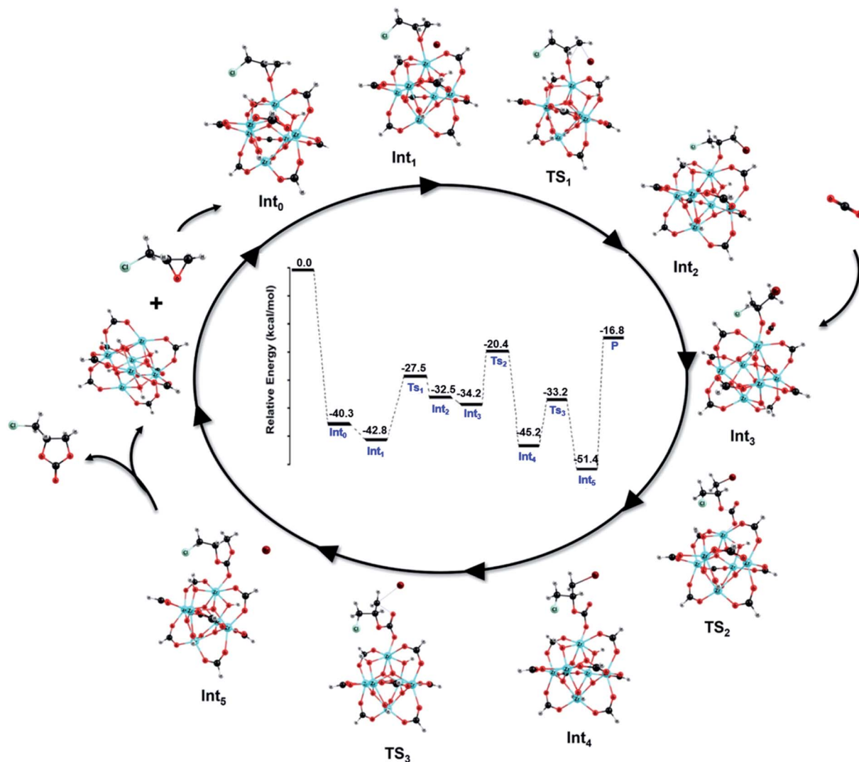
Fig. 8 Relative energy profile for the MOF-801/TBABr catalyzed cycloaddition reaction of \text{CO}_2 with ECH to form chloropropene carbonate and the DFT optimized structures of intermediates and transition states.
