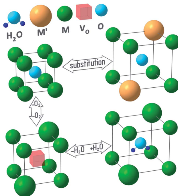
Fig. 1 Possible causes of chemical expansion of oxide materials, represented for a hypothetical M_{1-x}M'_xO_{1-y}(\text{H}_2\text{O})_z oxide.
