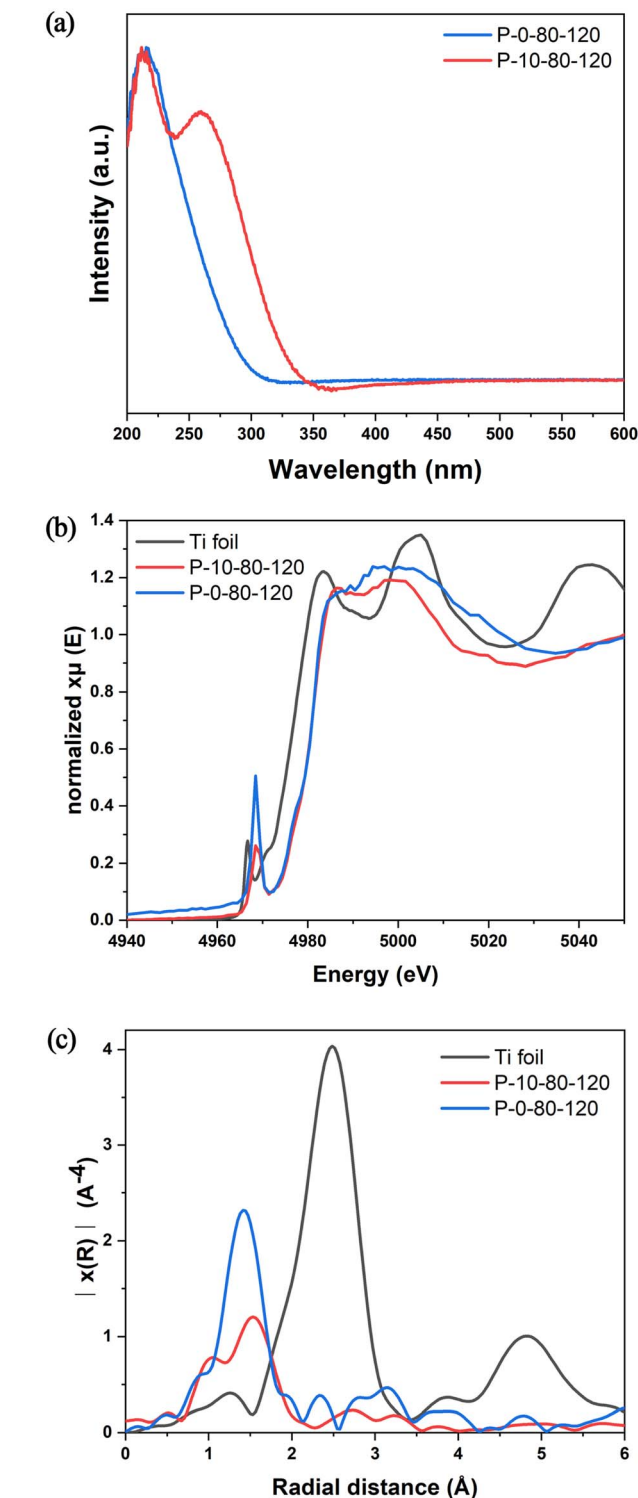
Fig. 4 (a) UV-vis spectra, (b) Ti K -edge XANES spectra, and (c) Fourier transform k^2 -weighted Ti EXAFS spectra in the R spacing of P-0-80-120 and P-10-80-120.
