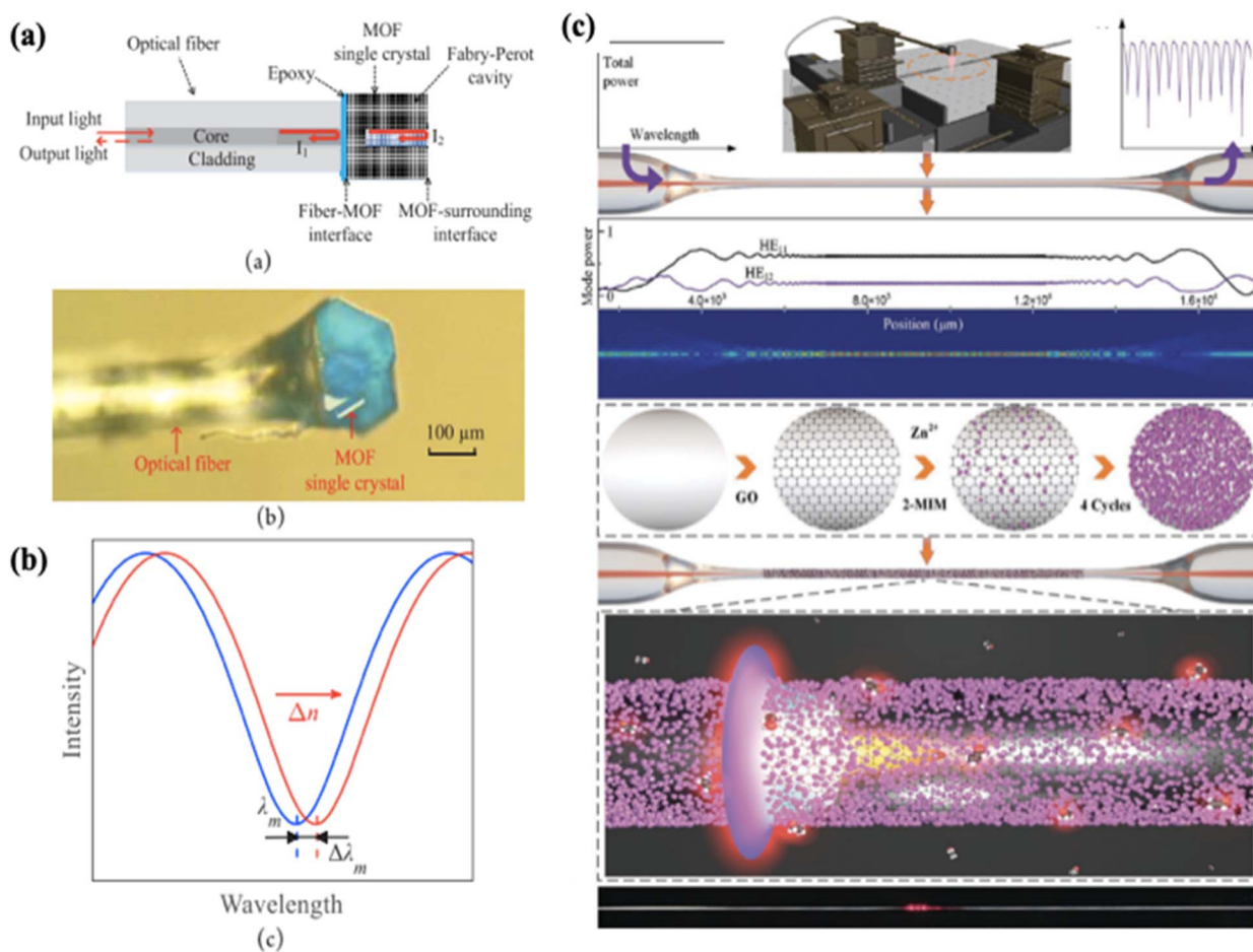
Fig. 12 (a) Schematic diagram of the HKUST-1 coated optical fibre sensor and an optical microscope image of the sensor. (b) Illustration of a section of the original (blue) and shifted (red) interferograms. 180 (c) Schematics of the modification step at the interface of the optical microfibre with a ZIF-8/GO functional layer. 118
