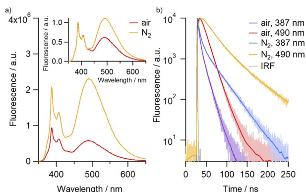
Fig. 2 (a) Emission spectra of 4Py in air-equilibrated (red) and N_2 -saturated (orange) MeCN ( 2.6 \times 10^{-6} M). Inset: the same spectra after normalization. (b) Fluorescence time profiles recorded with 4Py in air-equilibrated and N_2 -saturated MeCN at emission wavelengths corresponding to the emission from monomer (387 nm) and excimer (490 nm), including IRF (instrument response function). Smooth lines are the best fits of three-exponential global analysis.
