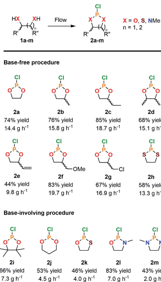
Fig. 2 Scope of cyclic adducts 2a–m obtained from the continuous flow reaction of PCl 3 with various diols and analogs through a base-free (see Table 1, entry 10) or a base-involving (see ESI, Section 2.5.2†) procedure.
