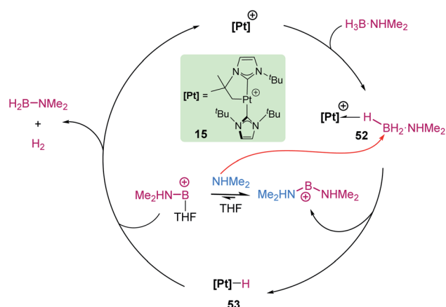
Scheme 61 Mechanism for the dehydrocoupling of \text{NMe}_2\text{H} \cdot \text{BH}_3 catalysed by 15 .
