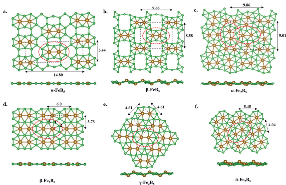
Fig. 3 Different optimized 2D monolayers derived from 10 : (a) \alpha - FeB_5 , (b) \beta - FeB_5 , (c) \alpha - Fe_2B_5 , (d) \beta - Fe_2B_5 (the numbering of three unique boron atoms is given in black, and Fe is denoted using red), (e) \gamma - Fe_2B_5 , and (f) \delta - Fe_2B_5 . Two different views of each monolayer are shown. Unit cells are indicated by the black dotted lines and lattice parameters are given in Å. Parent building blocks are highlighted using red dotted circles.
