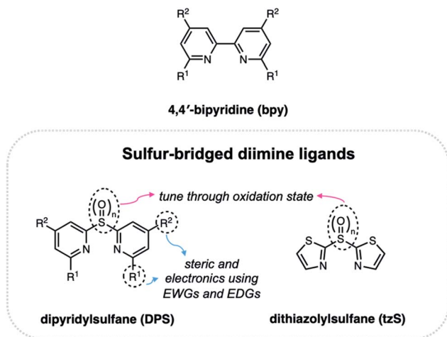
Fig. 15 Structure of 4,4'-bipyridine ligand (bpy) compared to sulfur-bridged diimine ligands based on dipyrldisulfane (DPS) and dithiazolysulfane (tzS).
