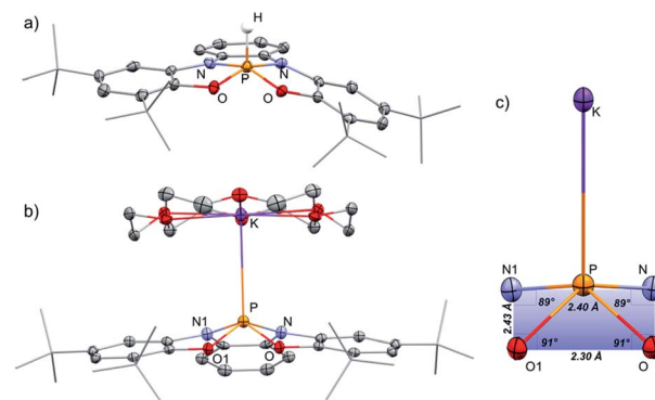
Fig. 2 POV-ray depiction of 1-H (a), [1^-][\text{K}(\text{18-crown-6})] (b), and the structural features of the SP fragment (c). Thermal ellipsoids at the 50% probability level, non-relevant hydrogens were omitted for clarity.
