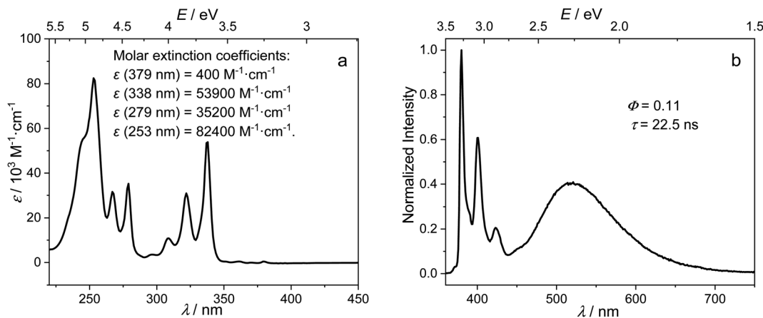
Fig. 2 Absorption (a) and normalized emission (b) excitation at 338 nm (3.67 eV) spectra of 1 in hexane at room temperature.
