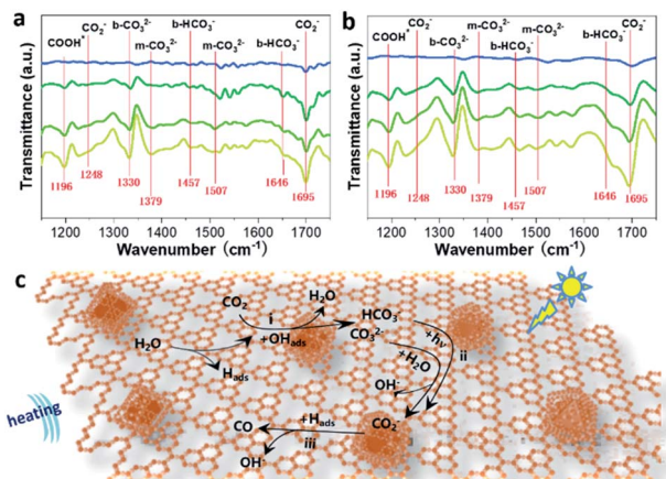
Fig. 4 In situ FTIR spectra of m-CN@CsPbBr 3 under (a) bare thermocatalytic and (b) photo-thermal conditions at ten-minute increments from 0 to 30 min (from top to bottom). (c) Schematic diagram of the possible reaction pathways of the CRR for the sample of m-CN@CsPbBr 3 under photo-thermal conditions.
