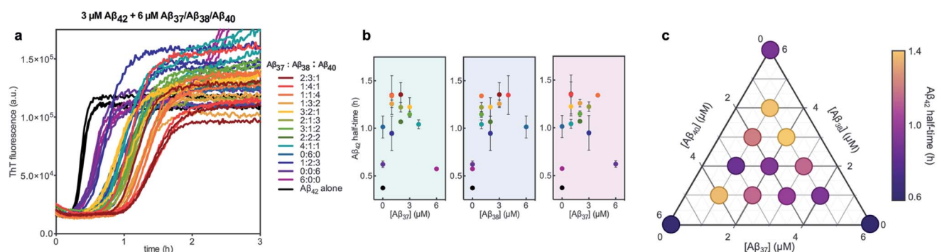
Fig. 12 Aggregation kinetics of 3 \mu\text{M} \text{A}\beta_{42} with 6 \mu\text{M} of \text{A}\beta_{37} / \text{A}\beta_{38} / \text{A}\beta_{40} mixtures in varying molar ratios. (a) The first ThT transition, corresponding to the aggregation of \text{A}\beta_{42} is shown; the full aggregation profiles are shown in Fig. S4†. (b) The half-times of \text{A}\beta_{42} aggregation in (a), versus the concentration of \text{A}\beta_{37} (green panel), \text{A}\beta_{38} (blue panel), and \text{A}\beta_{40} (red panel). The color of each point corresponds to the curves of the same color in (a). (c) Triangular heat-map representation of the half-time of \text{A}\beta_{42} aggregation depending on the \text{A}\beta_{37} / \text{A}\beta_{38} / \text{A}\beta_{40} concentrations. Experiments were performed in 20 mM sodium phosphate buffer, pH 7.4, with 200 \mu\text{M} EDTA, 0.02% \text{NaN}_3 , and 20 \mu\text{M} ThT.
