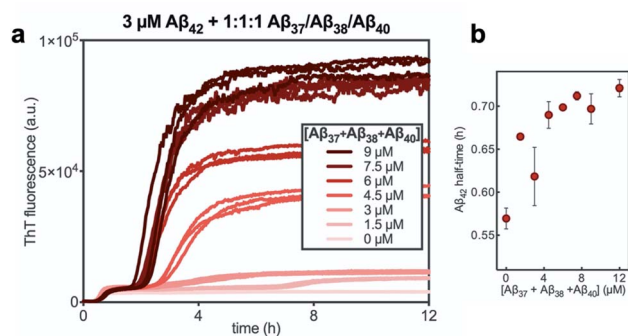
Fig. 11 (a) The aggregation of 3 \mu\text{M} \text{A}\beta_{42} with varying concentrations of a 1 : 1 : 1 mixture of \text{A}\beta_{37} / \text{A}\beta_{38} / \text{A}\beta_{40} . (b) The half-time of the aggregation of \text{A}\beta_{42} shown in (a) versus the total concentration of the three shorter alloforms. Kinetic experiment was performed in 20 mM sodium phosphate buffer, pH 7.4, with 200 \mu\text{M} EDTA, 0.02% \text{NaN}_3 , and 20 \mu\text{M} ThT.
