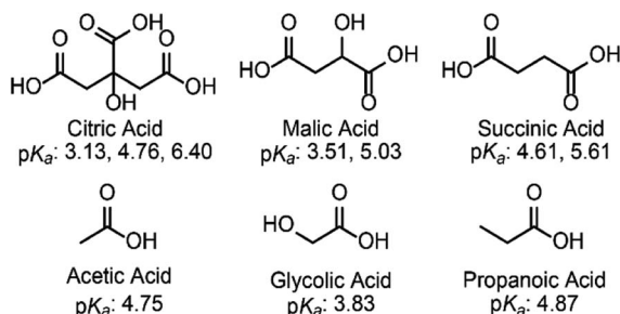
Scheme 1 Fully protonated structures and \text{p}K_{\text{a}} s of the acids discussed in this study.
