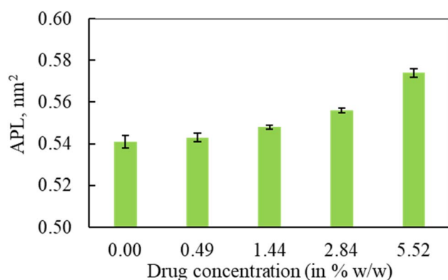
Fig. 6 The effect of hydrocortisone concentration on the area per lipid (APL) from the simulation of protein containing system at 20 \text{ mN m}^{-1} . The data were estimated over the last 1 \mu\text{s} of the 2 \mu\text{s} simulation. The error bar refers to standard deviations of the APL data across the frames.
