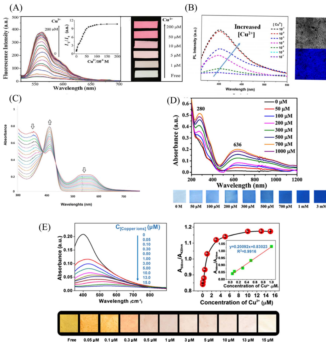
Fig. 4 Sensing properties of copper ion sensors prepared by chemical modification. (A) Reprinted with permission from ref. 85. Copyright 2013, The Royal Society of Chemistry . (B) Reprinted with permission from ref. 86. Copyright 2016, Elsevier. (C) Reprinted with permission from ref. 87. Copyright 2018, Elsevier. (D) Reprinted with permission from ref. 88. Copyright 2021, American Chemical Society . (E) Reprinted with permission from ref. 89. Copyright 2018, Springer-Verlag GmbH Austria, part of Springer Nature.
