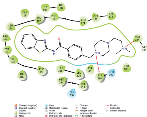
Fig. 7 2D interaction of compound 4f at binding region of MAO-B (PBDID: 2V5Z).
