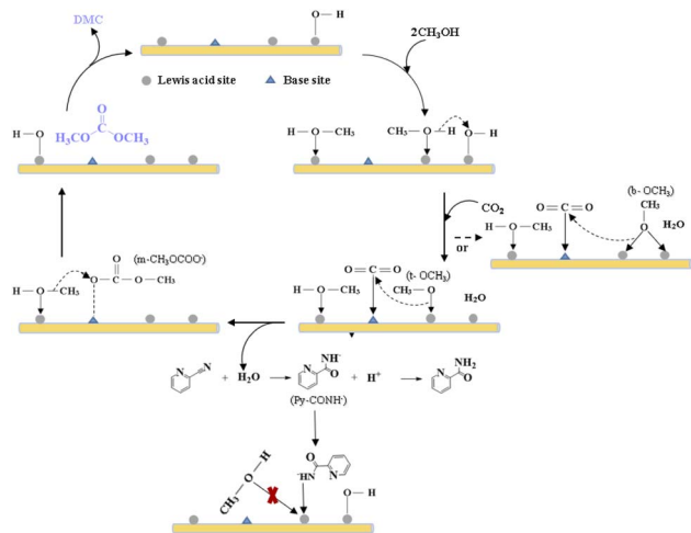
Scheme 2 Possible mechanism scheme for the catalytic CO 2 conversion into DMC over Ce-doped MOF.
