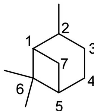
Fig. 1 IUPAC numbering of the pinene scaffold.
