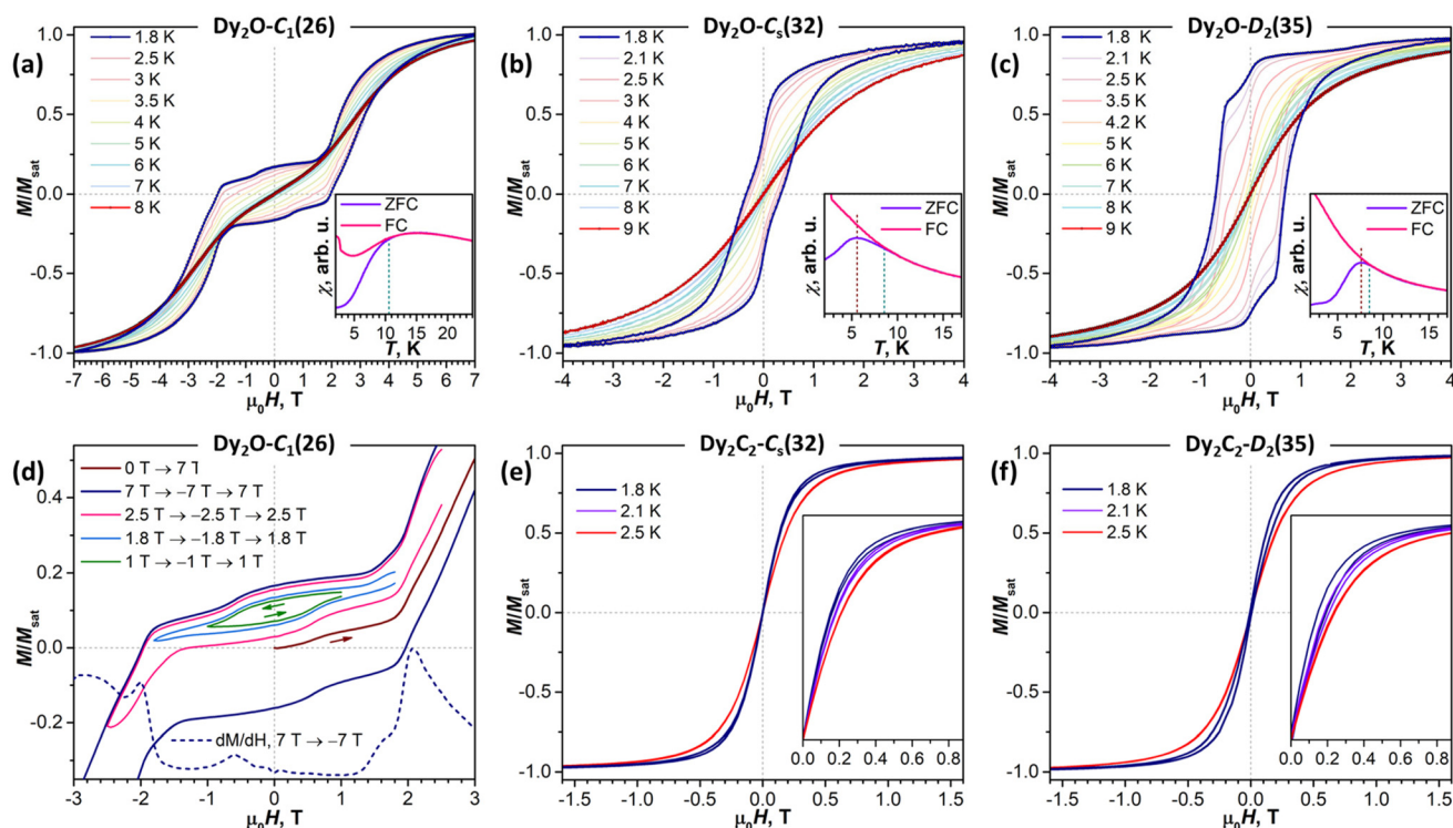
Fig. 7 Low-temperature magnetization curves of Dy 2 O@C 88 and Dy 2 C 2 @C 88 EMFs: Dy 2 O-C 1 (26) (a and d), Dy 2 O-C 5 (32) (b), Dy 2 O-D 2 (35) (c), Dy 2 C 2 -C 5 (32) (e), and Dy 2 C 2 -D 2 (35) (f), sweep rate 2.9 mT s -1 . Insets in (a)–(c) show \chi_{FC} and \chi_{ZFC} curves (0.2 T, sweep rate 5 K min -1 ) and determination of T_B and T_{irrev} . (d) Shows magnetic hysteresis of Dy 2 O-C 1 (26) measured in different field ranges at 1.8 K, as well as the derivative of the magnetization curve.
