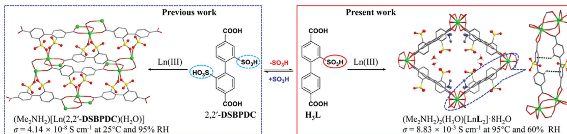
Scheme 2 The comparison of the MOFs built from 2,2'- DSBPDC and H 3 L .
