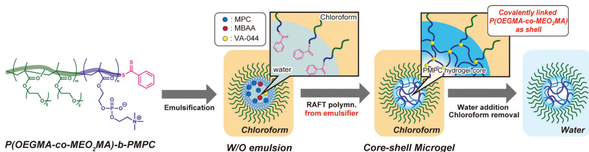
Fig. 1 Schematic illustration of the preparation of PMPC core-shell microgels by inverse miniemulsion RAFT copolymerization of MPC and MBAA using water-soluble P(\text{OEGMA-co-MEO}_2\text{MA})\text{-}b\text{-PMPC} emulsifier.
