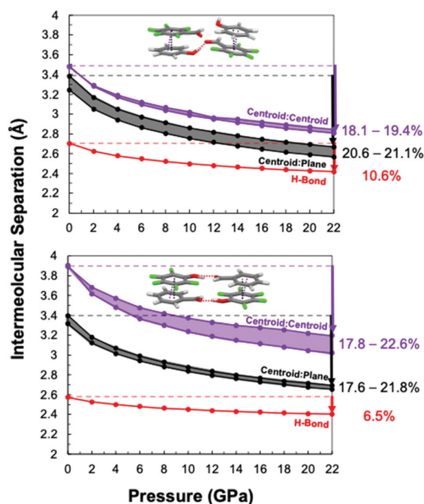
Fig. 2 Measured intermolecular interactions of simulated compressed co-crystals up to 22 GPa. Distances include centroid:centroid d_c (purple), centroid:plane d_p (black), and intra-stack O...O hydrogen bonding (red) of each co-crystal ArOH:ArFCHO (top) and ArCHO:ArFOH (bottom).
