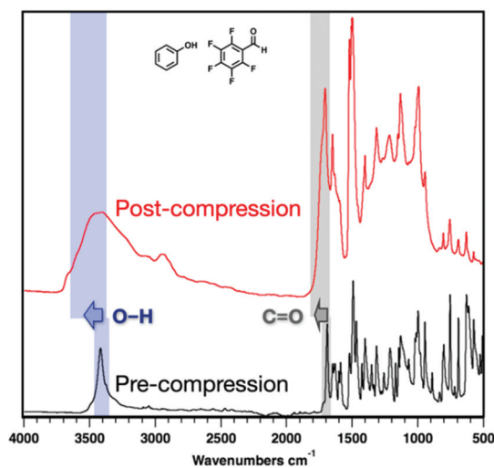
Fig. 5 IR spectrum of precursor ArOH:ArFCHO co-crystal prior to compression (black, bottom) and polymer after compression (top, red), featuring the shift to higher wavenumbers of both the -\text{OH} and \text{C}=\text{O} stretching.
