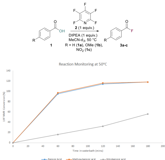
Fig. 1 Graph of conversion of benzoic acids to acyl fluorides. Reactions were conducted in NMR tubes in a thermostatically controlled water bath. 19 F NMR spectra were recorded at various time points using fluoro-benzene as an internal standard. Integration of the internal standard vs. integration of the acyl fluoride resonance was used to determine conversion.
